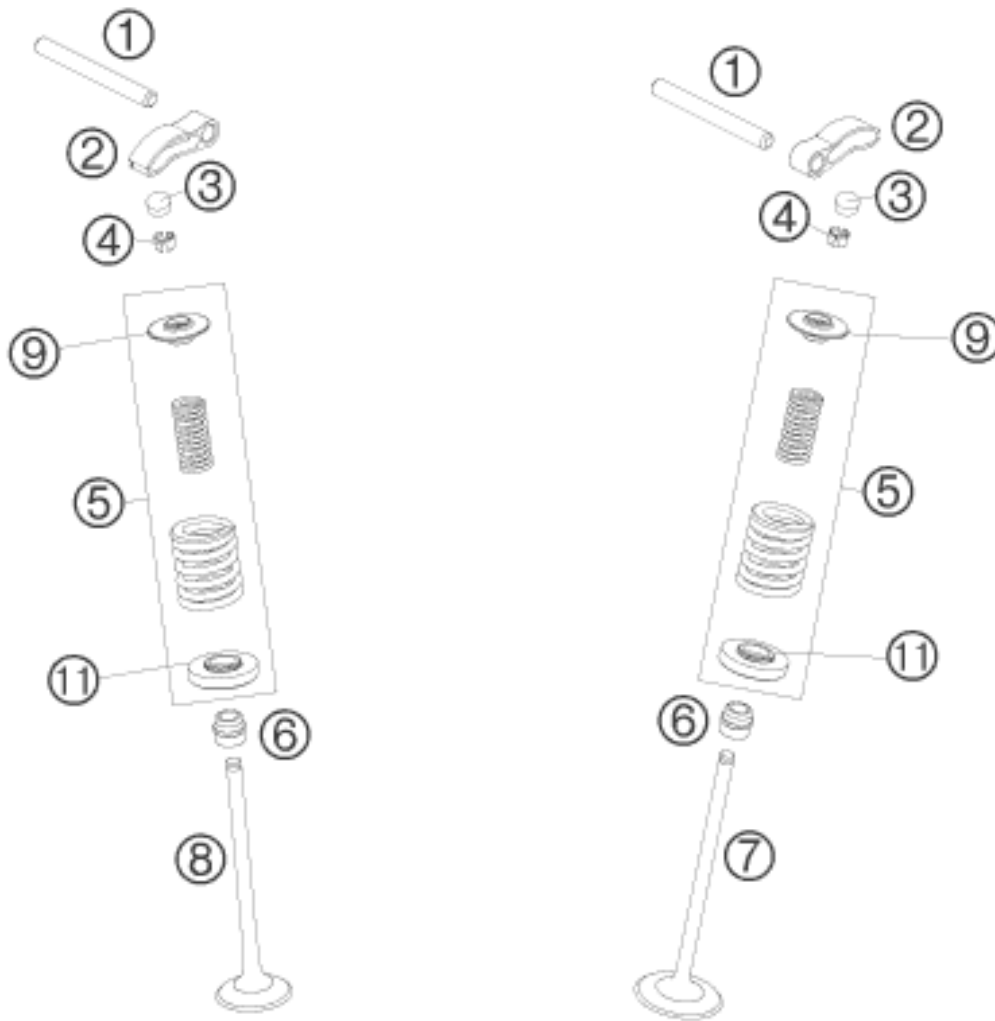
EXHAUST
